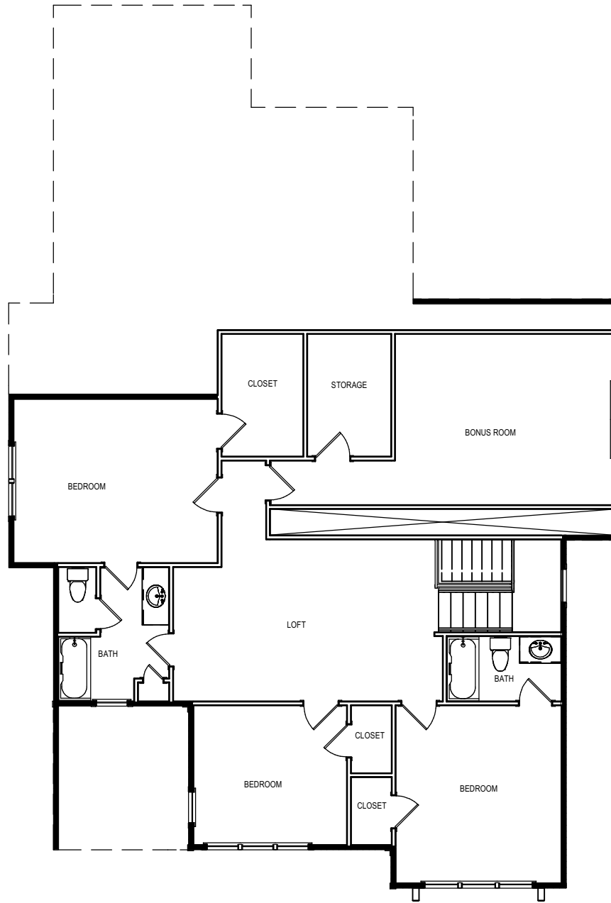
2ND FLOOR
