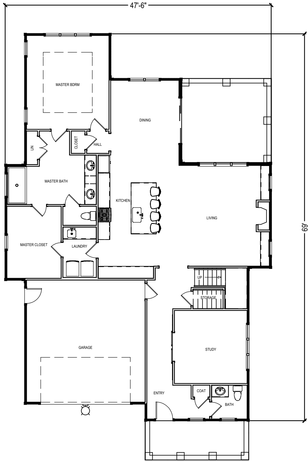
1ST FLOOR
